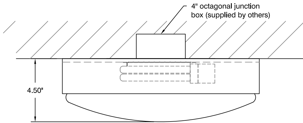
SIDE VIEW
