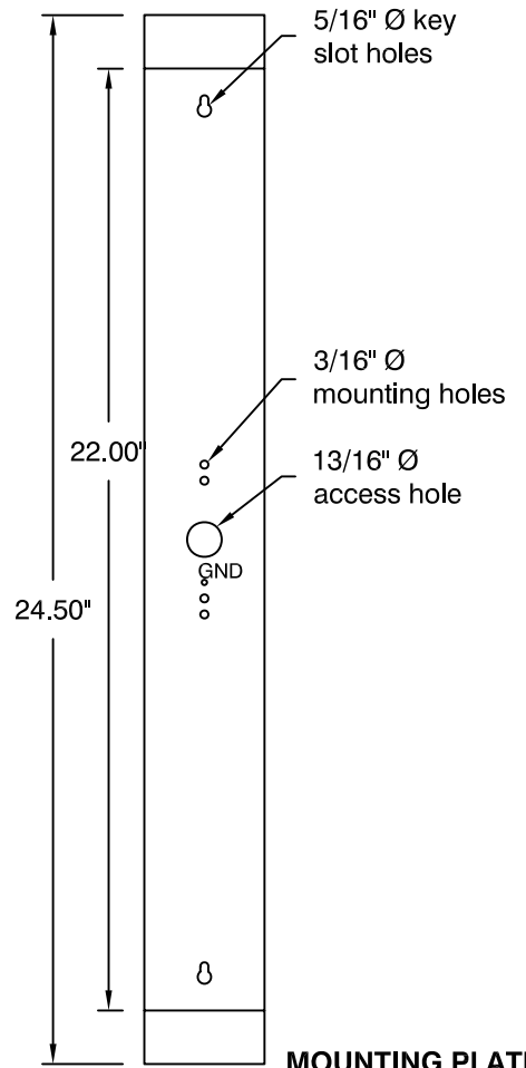
MOUNTING PLATE
