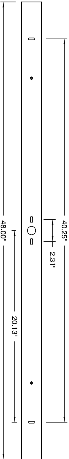
FRONT VIEW
