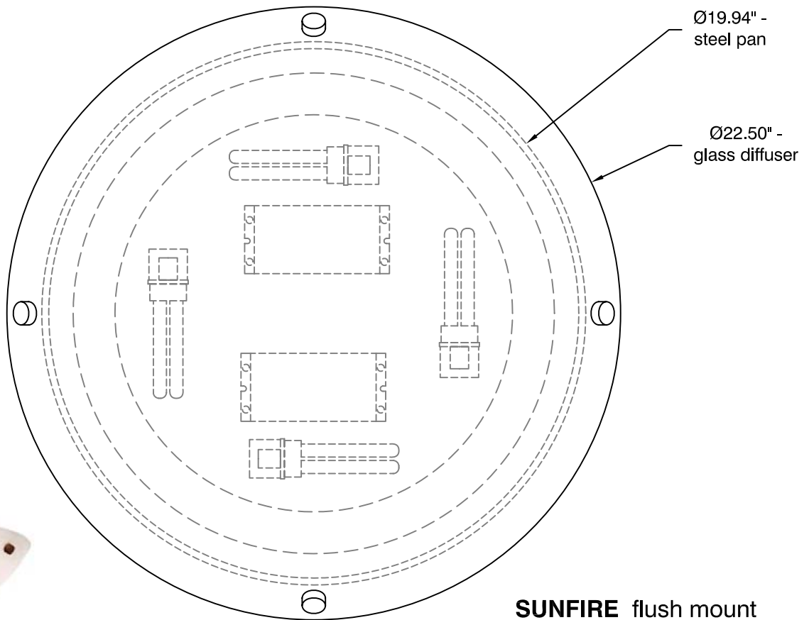
BOTTOM VIEW
