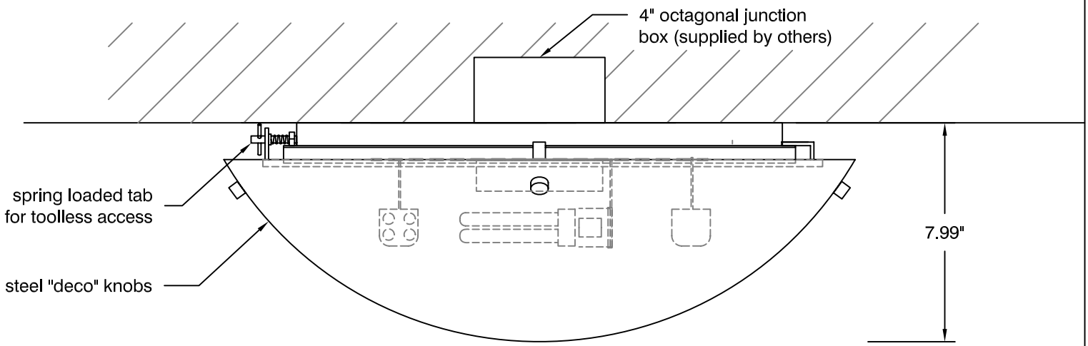
FRONT VIEW
