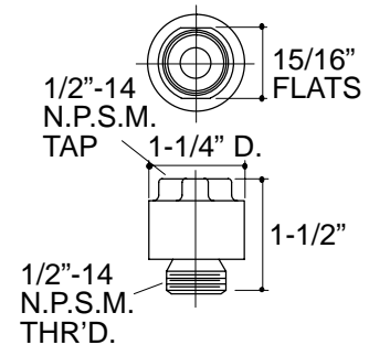
ELBOW AND VACUUM BREAKER DETAILS
