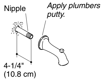
Threaded Spout
