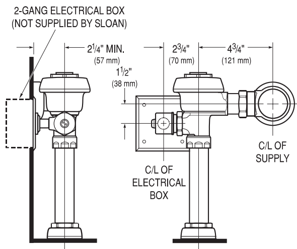
Typical Exposed “ES” Flushometer installation (Water Closet or Urinal).
