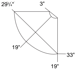
1702-90 Corner 90° Hang Table
