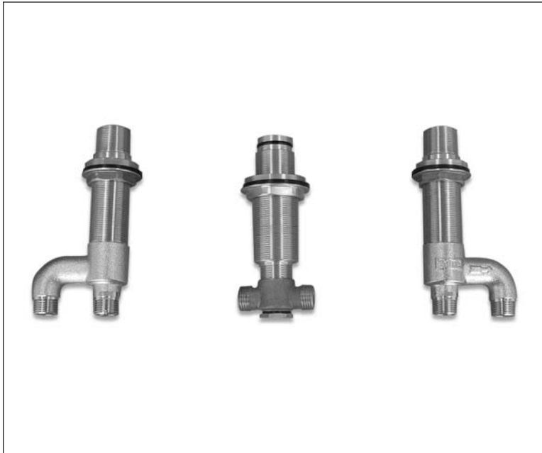
TB6T - Deck-Mounted Bath Faucet Valve (1/2")
