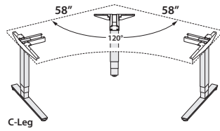
TLCZ-5858-NNNNCPB
