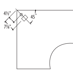
Corner Worksurface
