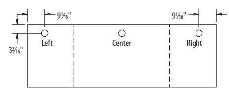
18" and 24" deep Worksurfaces
