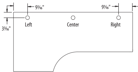
Extended Corner Worksurface (Right shown)
