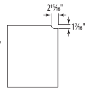
Pedestal
