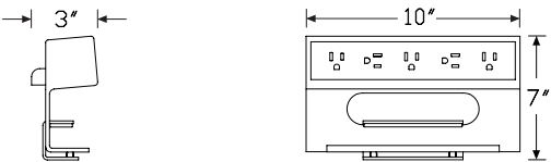
5 simplex receptacles
