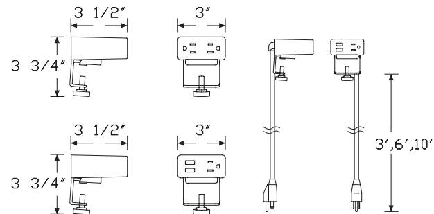
Surface Clamp
