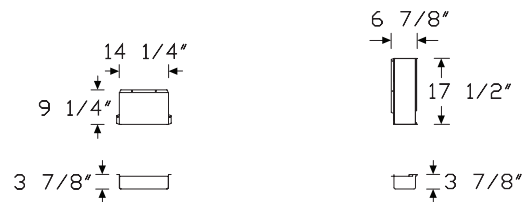
Jumper Tray (00)
