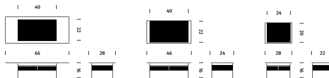
Layer Occasional Table with Drawer
