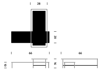
Layer Occasional Table, Nesting
