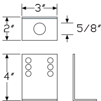
B - for use with 5/8" anchor
