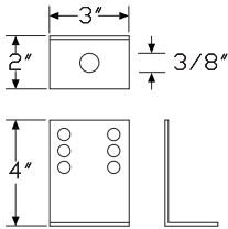
A - for use with 3/8" anchor
