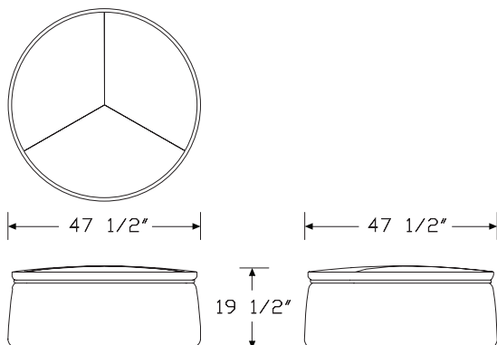
3-Seat Stool
