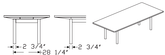
Leg Type A - Post Leg
