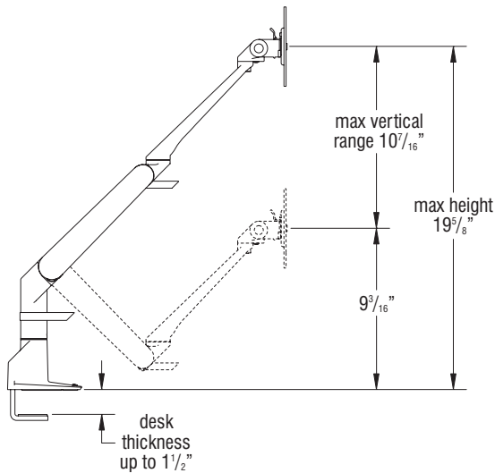
Side View - Vertical Range
