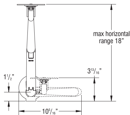
Top View - Horizontal Range & Arm Folded
