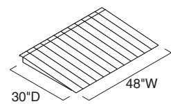
Ramp Kit
