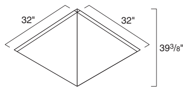
Corner Ramp
