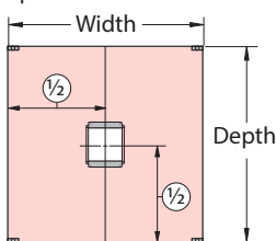
14" x 14" Cable Base
