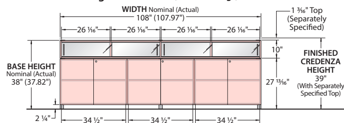
Front View – 39" High x 108" Wide (6 Doors/6 Legs)
