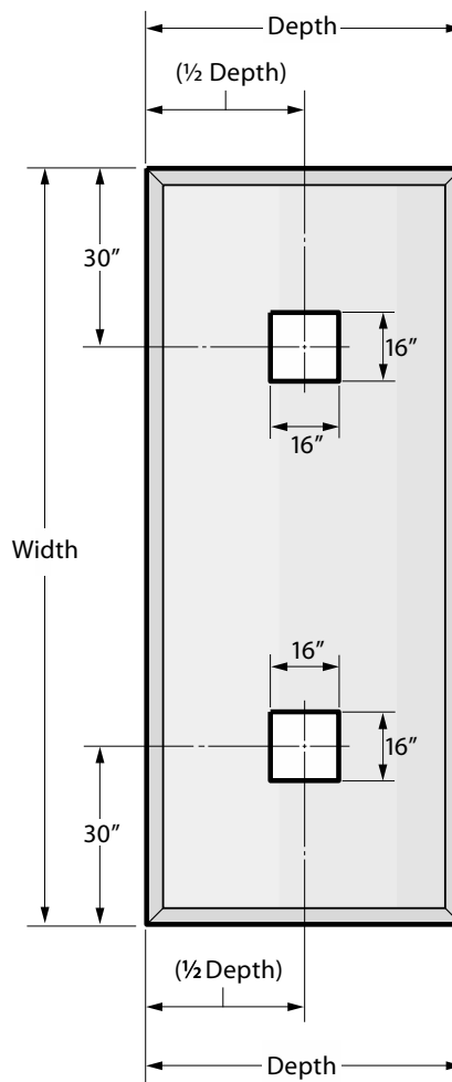
Top View with (2) Cutouts
