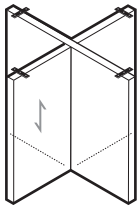
X Base 1 1/4" Thick 26", 32" Lengths
