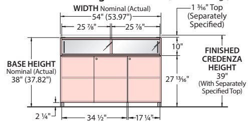
Front View – 39" High x 72" Wide (4 Doors/6 Legs)
