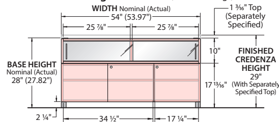
Front View – 29" High x 72" Wide (4 Doors/6 Legs)
