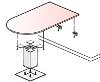
Square Column Base Plate (Optional)
