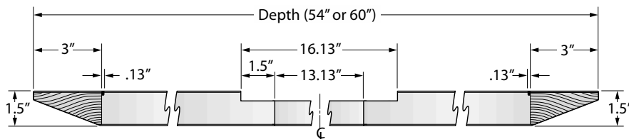
Section/Side View – Cutout Location /Edge Detail
