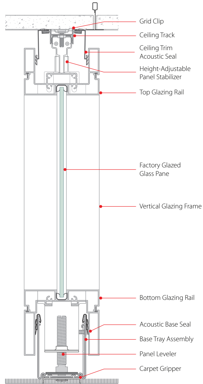
VERTICAL SECTION
