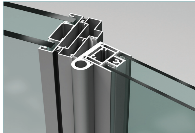
COMPRESSION SEALS
