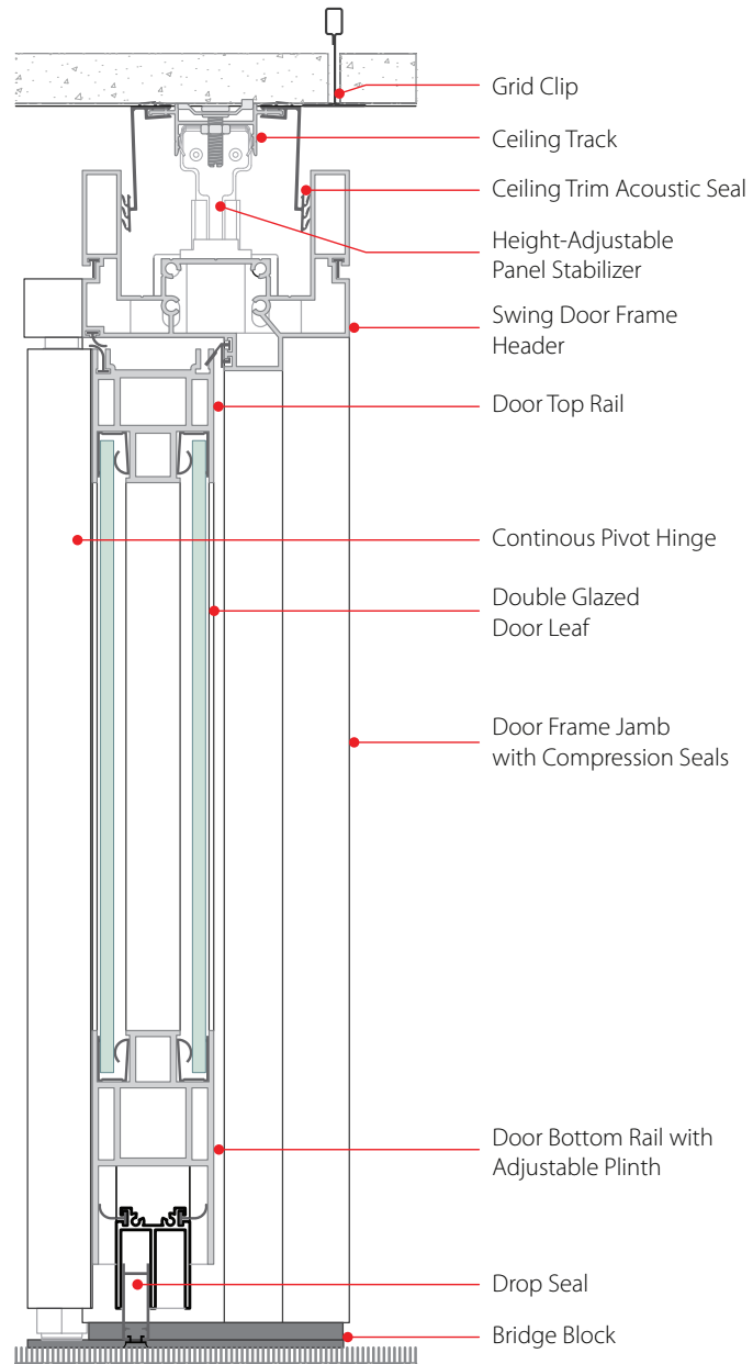
VERTICAL SECTION
