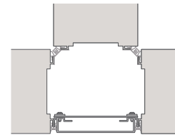
3-WAY 90°
