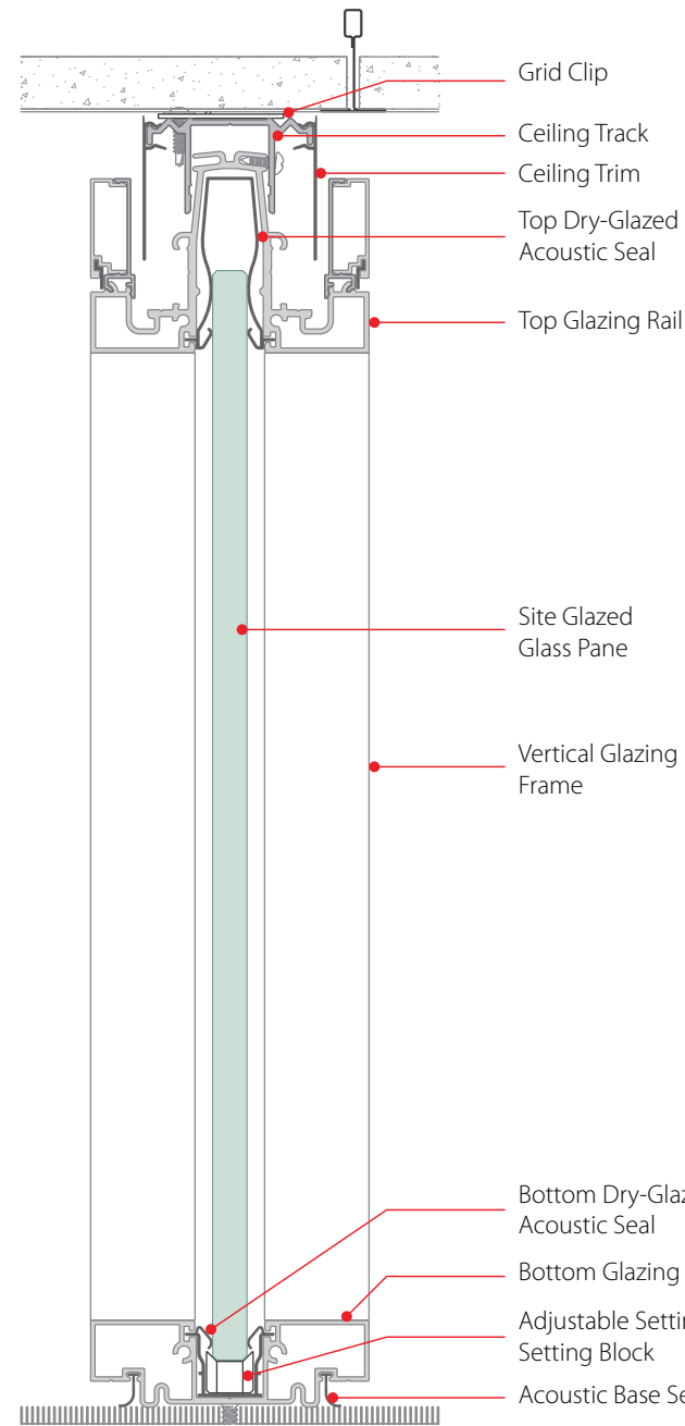
VERTICAL SECTION
