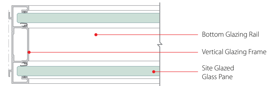
HORIZONTAL SECTION
