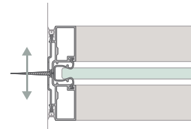
OFF-MODULAR T-MOUNT
