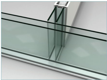
DOUBLE GLAZED TO DOUBLE GLAZED
