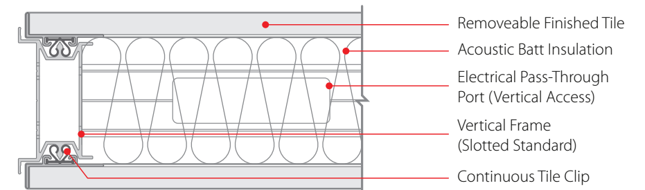
HORIZONTAL SECTION
