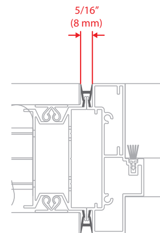
SOLID WALL TO SWING DOOR FRAME VERTICAL REVEAL
