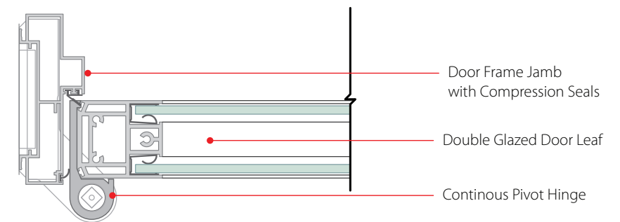
HORIZONTAL SECTION
