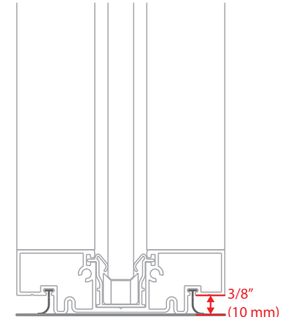
FRAMELESS GLASS FLOOR SHADOWGAP
