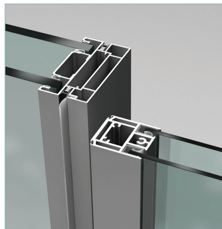
INTEGRATED STRIKE + BYPASS SEALS
