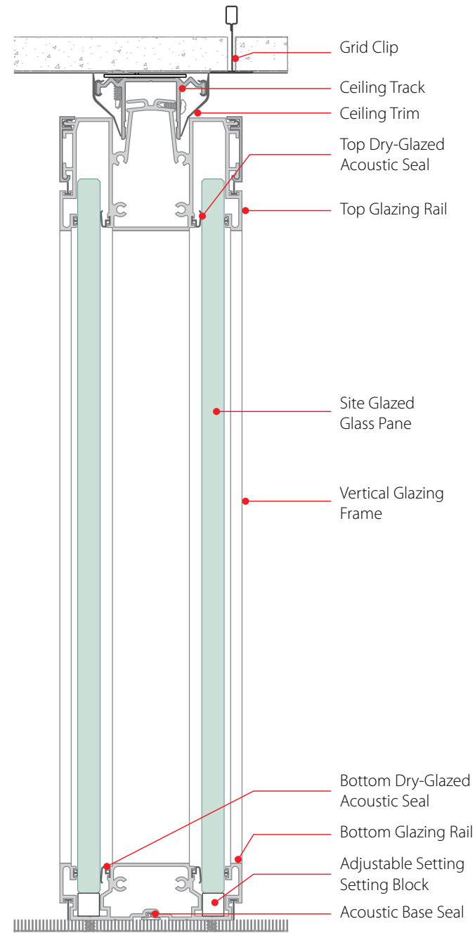
VERTICAL SECTION
