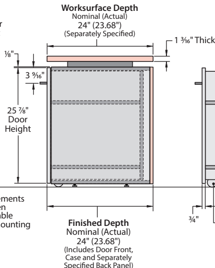
Side View (Closed Position)
