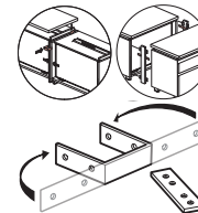
Ganging Bracket Kit QAGB-0000
