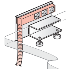
Power Tap – Horizontal and Power Tap Bracket Adjustable
