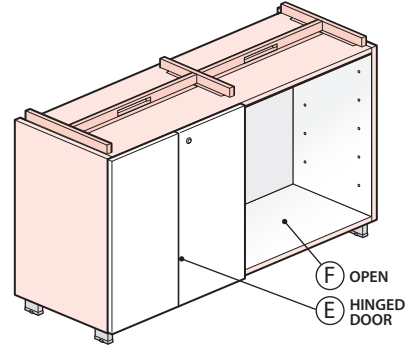
Two-High Hinged Door (Left) – Open (Right) QBDF-29XX-JZN Alternative Configuration: Open (Left) – 24" Hinged Door (Right) QBDF-29XX-ZJN
