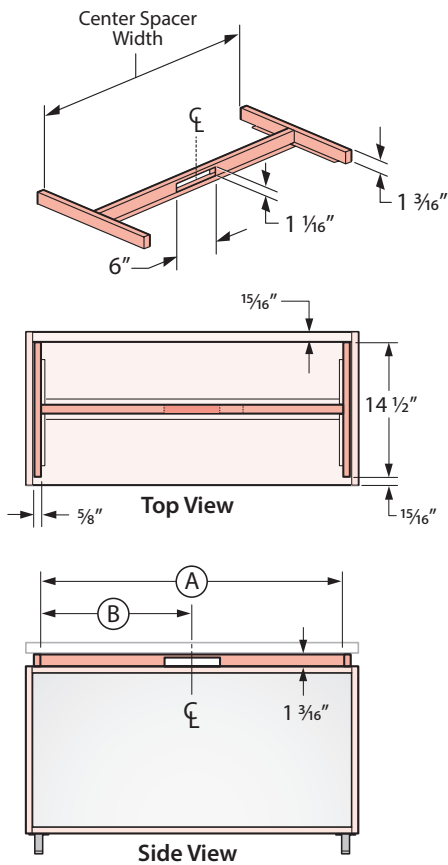
24", 30", 36" and 42" Wide Base Units (Single Width)
