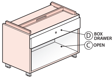
One and One-Half High Box Drawer/Open QBSF-23XX-CNN
