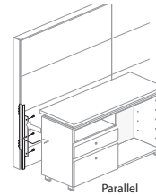
Storage to Panel Bracket – Parallel ZEBQ (UniGroup Too) ZZBQ (Compose) ZNBQ (PREMISE)
