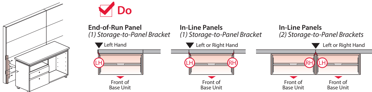
Parallel to Panel Storage-to-Panel-Bracket – Left Hand
