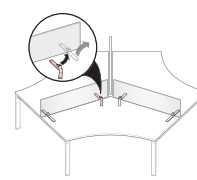
Bracket – Screen – For use with 120° Reside worksurface SUCB-0000
