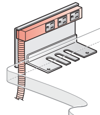
Power Tap – Horizontal and Power Tap Bracket Fixed
