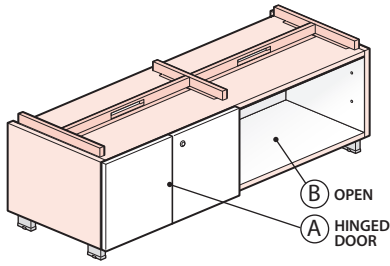
One-High Hinged Door (Left) – Open (Right) QBDF-17XX-GZN Alternative Configuration: Open (Left) – 12" Hinged Door (Right) QBDF-17XX-ZGN
