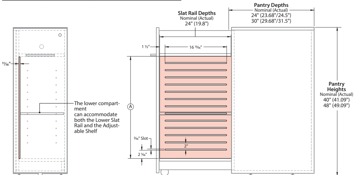
Accessory Slots Accommodate Separately Specified Belong Accessories
