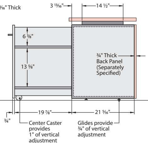
Side View (Open Position)
