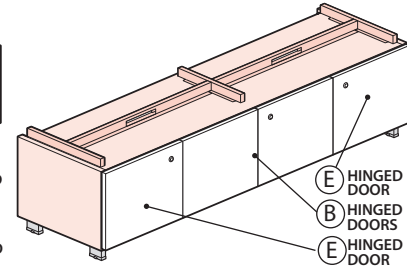
One-High Hinged Door (Left) – Hinged Door (Center) – Hinged Door (Right) QBTF-17XX-GGG
