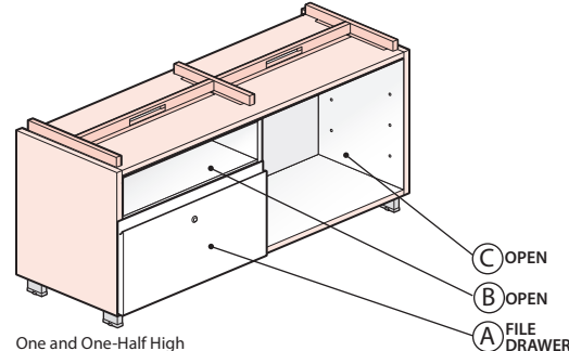
One and One-Half High Open/File Drawer (Left) – Open (Right) QBDF-23XX-DZN
