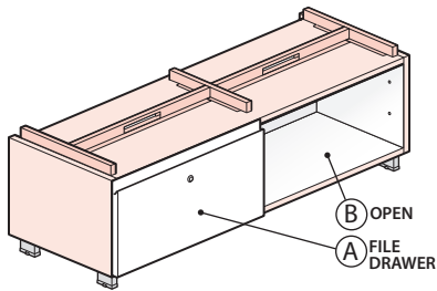
One-High File Drawer (Left) – Open Storage (Right) QBDF-17XX-AZN
