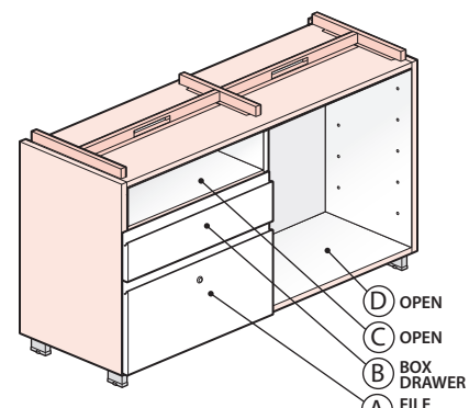
Two-High 6" Open/Box Drawer/File Drawer (Left) – Open (Right) QBDF-29XX-FZN
