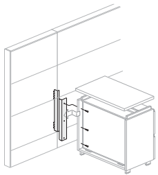
Right-Hand bracket Perpendicular application Z()BQ-RE
