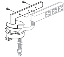
Power Tap – Horizontal and Power Tap Bracket with Grommet – Horizontal
