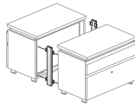
Filler Panel – One and One-Half High QAFF-0023-AL (1.5" Gap) QAFF-0023-BL (2.8" Gap) QAFF-0023-CL (5.1" Gap)
