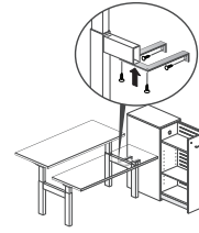
Planes Height Adjustable Table-Bench Bracket
