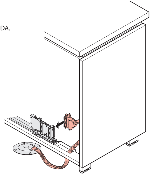
Infeed Harness Application
