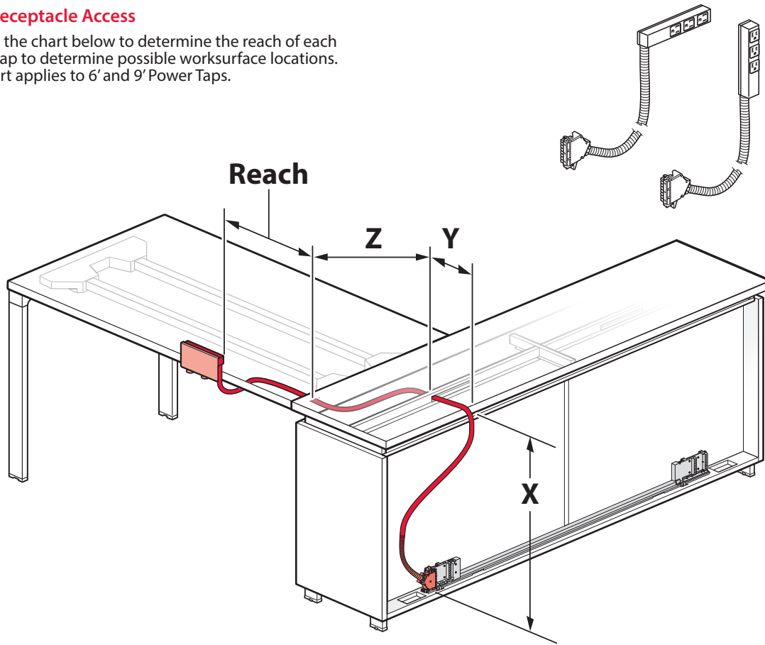
Reach (Adjustment Range of Power Tap from the edge of the Worksurface)
