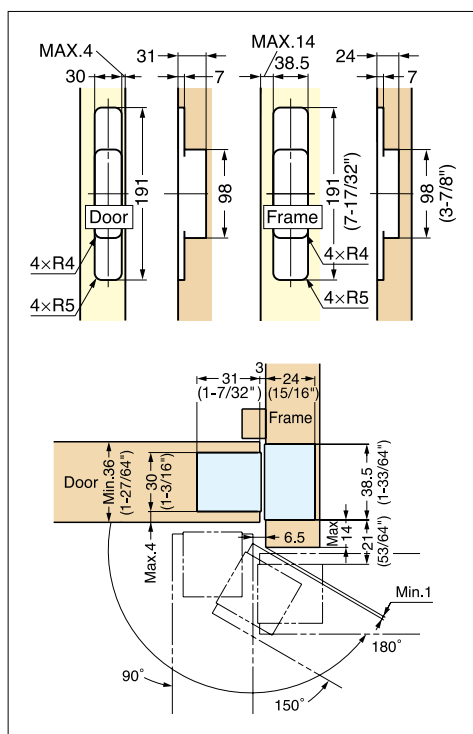
Bore Dimensions
