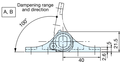
(W/Damper)
