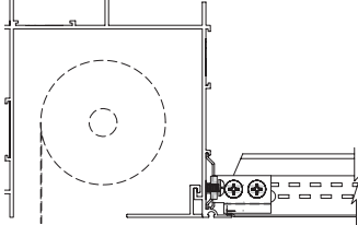
3-sided Axiom Perimeter Pocket, Acoustical/Drywall Transition with Axiom Perimeter Closure Clip 3"
