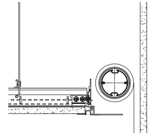
Pocketless Shade Options
