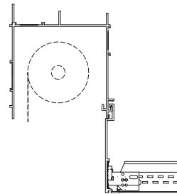
3-sided Axiom Perimeter Pocket, with 4" extension
