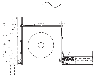
3-sided Axiom Perimeter Pocket
