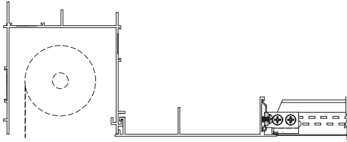
3-sided Axiom Perimeter Pocket, Connection to Extension/Face Plate with 7" Axiom Perimeter Face Plate
