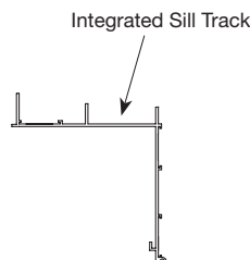
2-sided Axiom Perimeter Pocket
