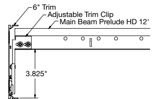
Adjustable Trim Clip (7239) in inverted position
