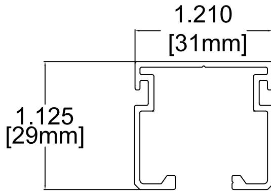
SECTION VIEW: CE80954 & CE80954-AN (not to scale)
