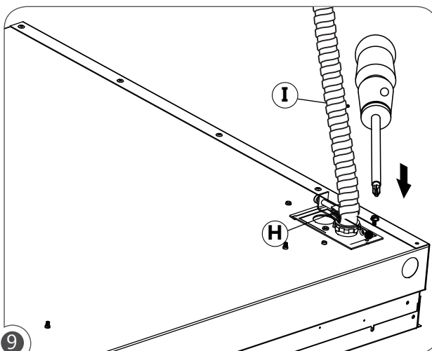
9 Push connected wires and wire nuts into fixture. Reinstall knockout plate (H) onto fixture by hooking tab into hole, and refastening screw to knockout plate (H) and fixture.
