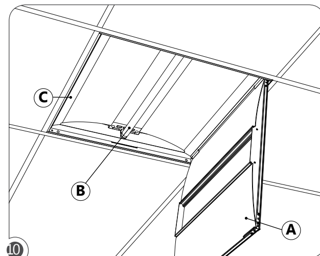
10 Reinstall lamps (B). Close the fixtures door (A). Power to the fixture (C) can now be safely turned on. Re-install the remaining tile to close the ceiling.
