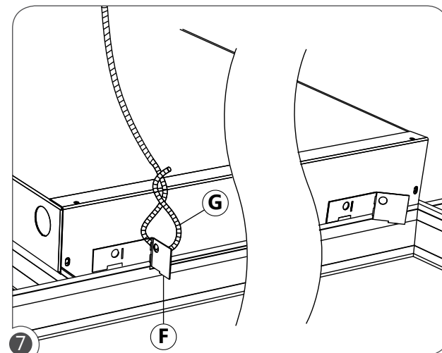
7 For additional safety a security wire (G) can be attached from the security tabs (F) to the structure above.
