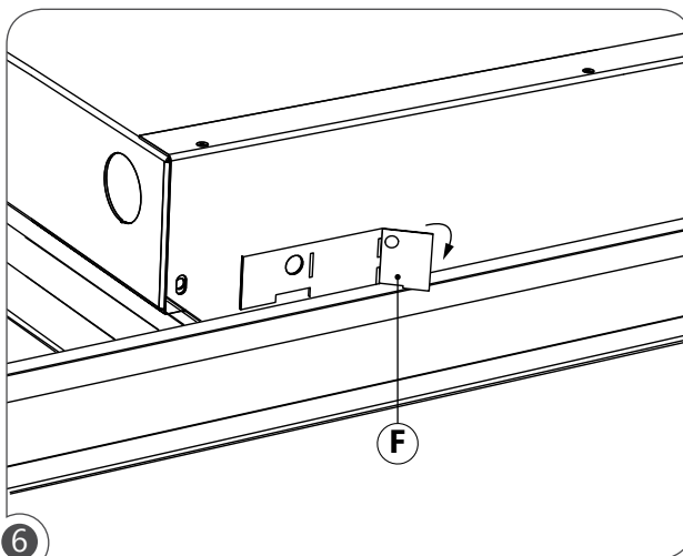
6 Based on ceiling type (tegular / screw slot T-bar or standard T-bar) bend a security tab (F) on each corner of the fixture to provide support. (SEE T-BAR STYLE MOUNTING pg.1).
