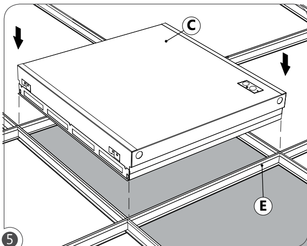
5 Set the fixture (C) into the T-bar grid (E).
