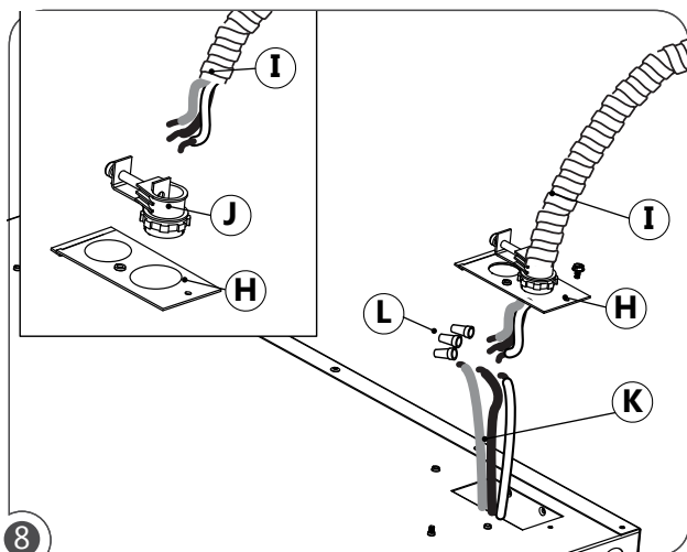
8 Remove knockout plate (H) and install BX connector (J) through the knockout plate (H). Insert BX cable (I) into BX connector (J) and fasten by tightening screw. Connect wires from BX cable (I) to wires on ballast (K) by using wire nuts (L). Ensure connections comply with local and national electrical codes.
