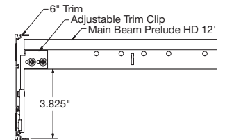
Adjustable Trim Clip (7239) in inverted position
