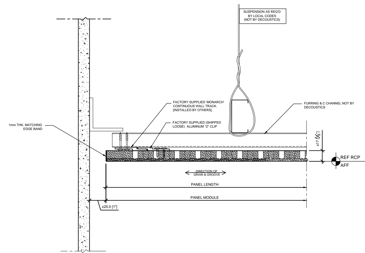
DETAIL @ STARTER PANEL SCALE: 1/2 REF.
