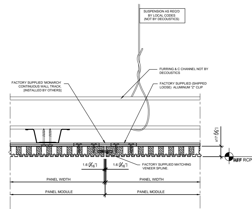
DETAIL @ DEFINED JOINT SCALE: 1/2
