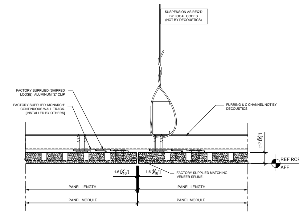
DETAIL @ DEFINED JOINT SCALE: 1/2
