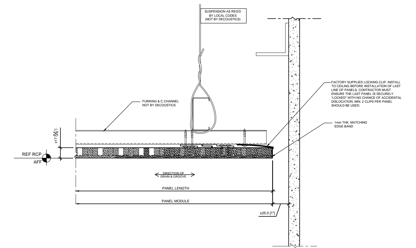
DETAIL @ END PANEL SCALE: 1/2 REF.
