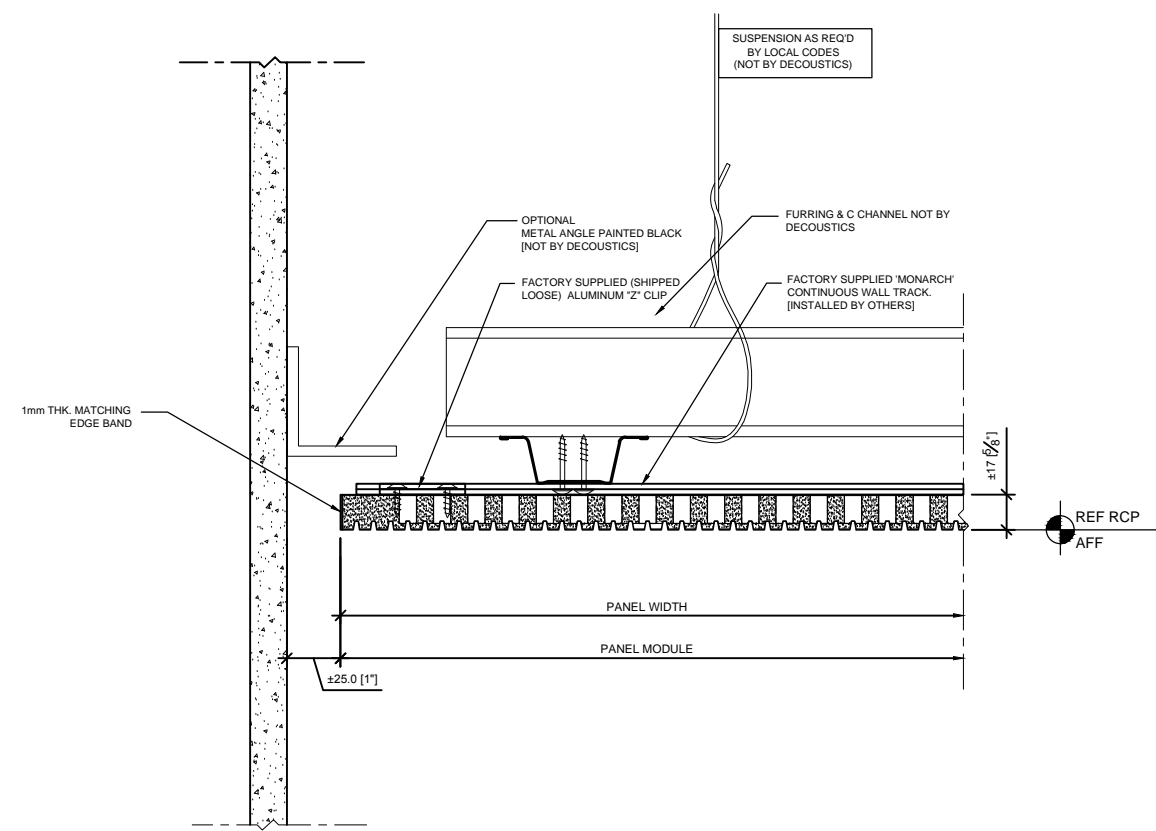
DETAIL @ PERIMETER (PERPENDICULAR TO GROOVES) SCALE: 1/2 REF.
