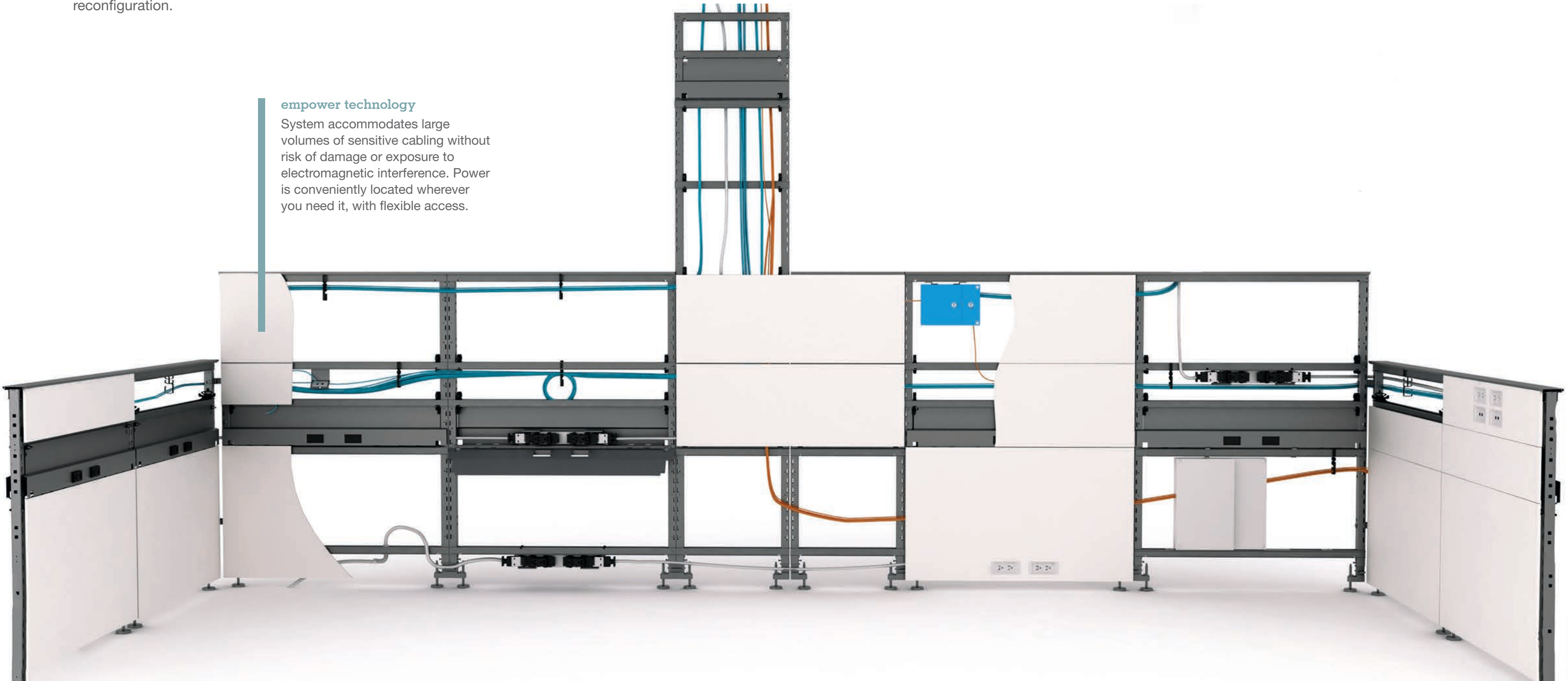
Lay-in technology, versus aperture-based systems, decrease install time - no need to thread cables through cut-outs in frames, saving time and manpower.
