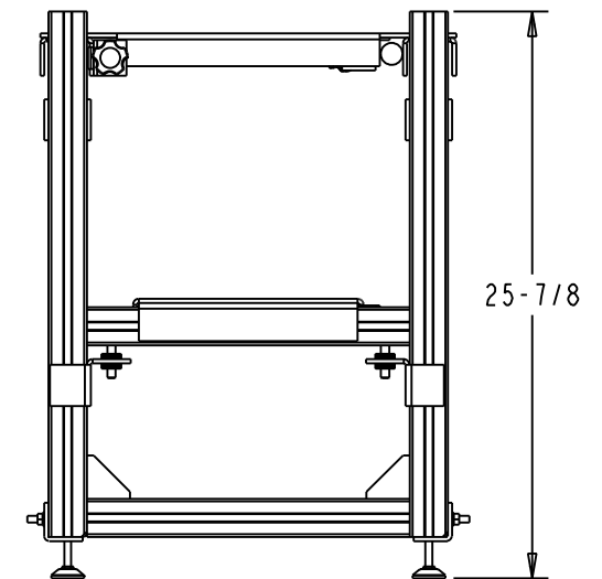
ELEVATION VIEW
