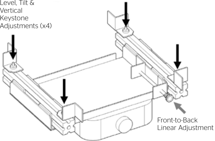
Bottom Projector Plate
