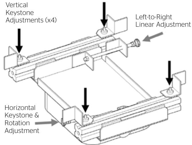
Top Projector Plate
