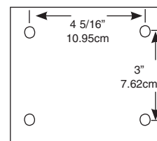
Mounting Bolt Pattern
