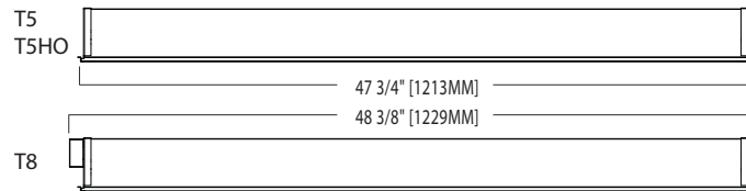
Alternate Dimensions - 2x4
