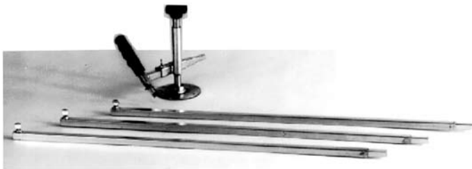
T204 Circle Maker & Extensions: Used to scribe or groove circles from 6" to 19' 6" in diameter in vinyl and linoleum products. Three extension poles are included. The Circle Maker can be fitted with a scribe pin, scribe blade, groover blade or slotted carpet knife blade (pins and blades not included).
