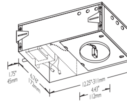
DHX-I HOUSING
