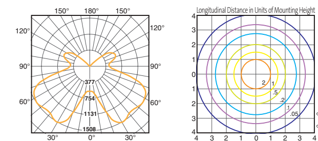
SAMG-MR-1-H175 (Type V Semi-Cutoff/mounting ht. = 16')
