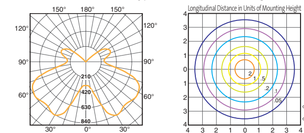
SAMG-MR-1-H175 (Type V Semi-Cutoff/mounting ht. = 16')
