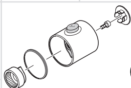
Ecostat 1001 96217XXX
