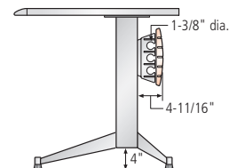
End Elevation View
