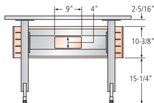
Side Elevation View
