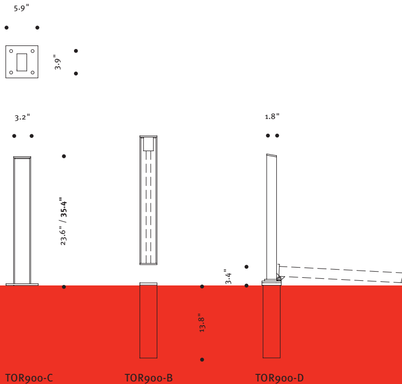
Flange Mount
