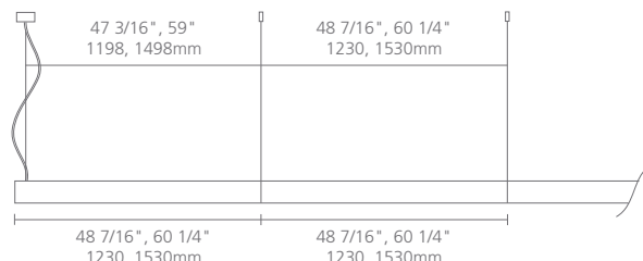
LINEAR LIGHTING SYSTEM
