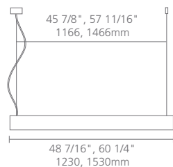
SINGLE SUSPENSION
