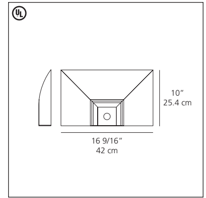
Flap wall (indirect + direct)
