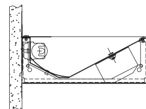
EXPOSED MOUNTING
