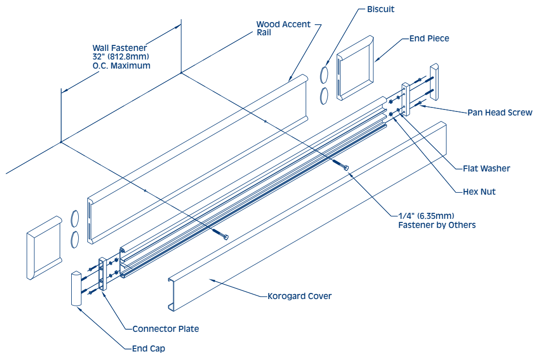
ASSEMBLY DRAWING
