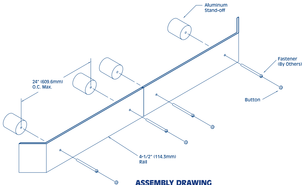
ASSEMBLY DRAWING
