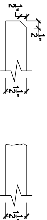
PROFILE 4: BEVEL
