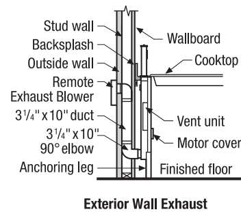
Exterior Wall Exhaust
