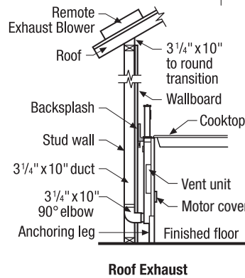
Roof Exhaust
