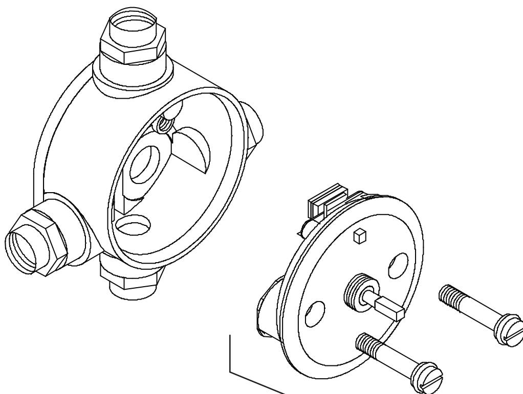
P11001-00-0 Thermostatic Valve Cartridge Assembly
